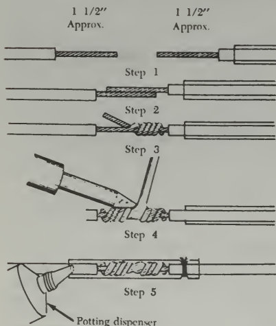
FIGURE 4-111. Repairing broken wire by soldering and potting.
